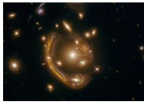
A Hubble Space Telescope image shows one of the most complete Einstein rings scientists have studied to date
