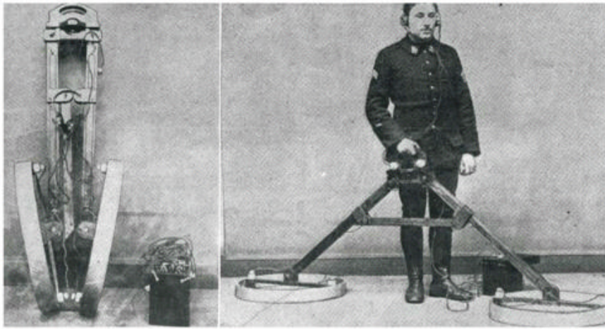
This is one of the first metal detectors. It was used in World War I to locate bombs
