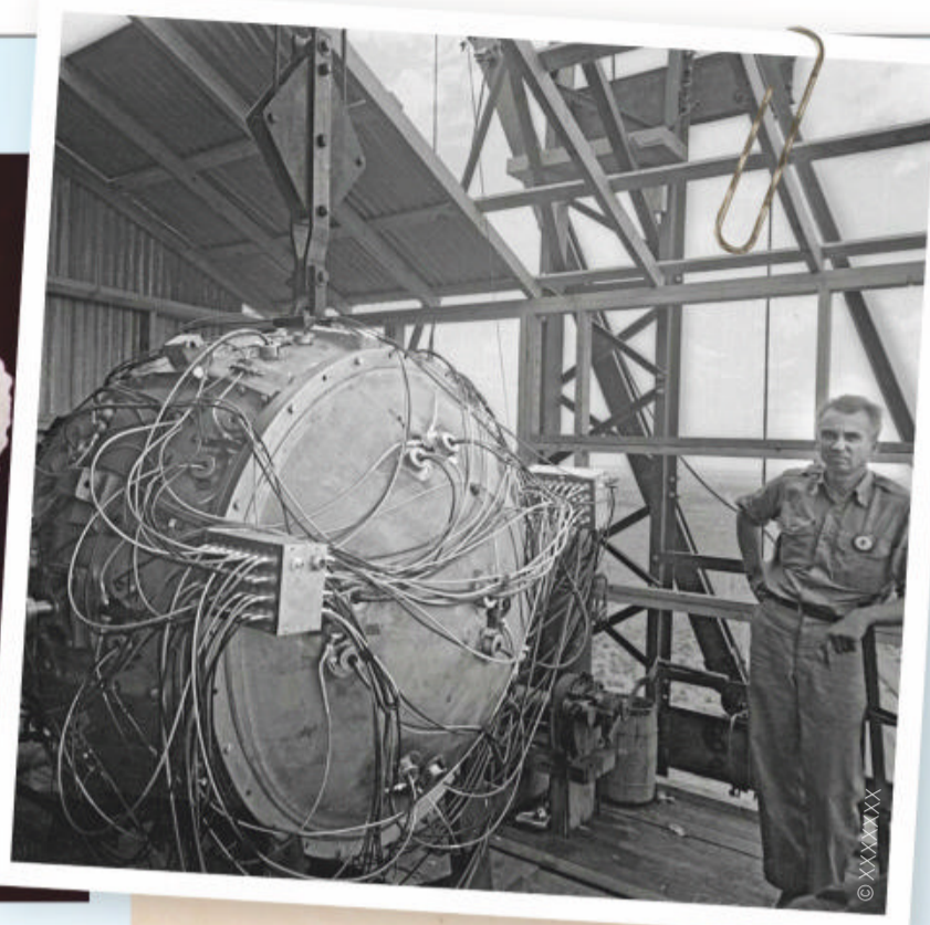
The 'Gadget' was a plutonium device, similar in design to the Fat Man bomb that was later dropped on Nagasaki, Japan
