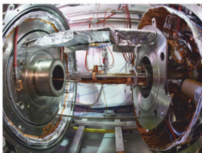
A magnetic ‘trap’ inside CERN’s antimatter factory, capable of storing antihydrogen atoms
