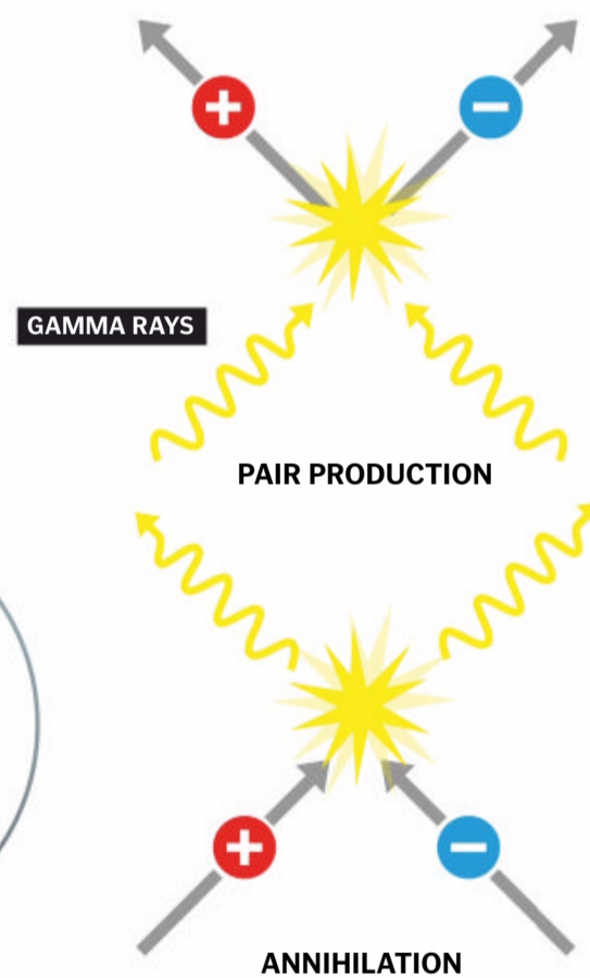
An electron-positron pair can appear spontaneously with enough energy, or annihilate, producing the same energy
