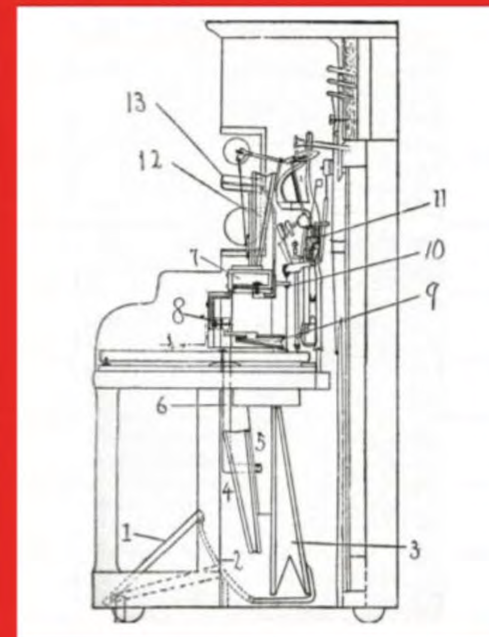
Pianolas rely on a series of valves and membranes to strike keys when triggered by an influx of air
