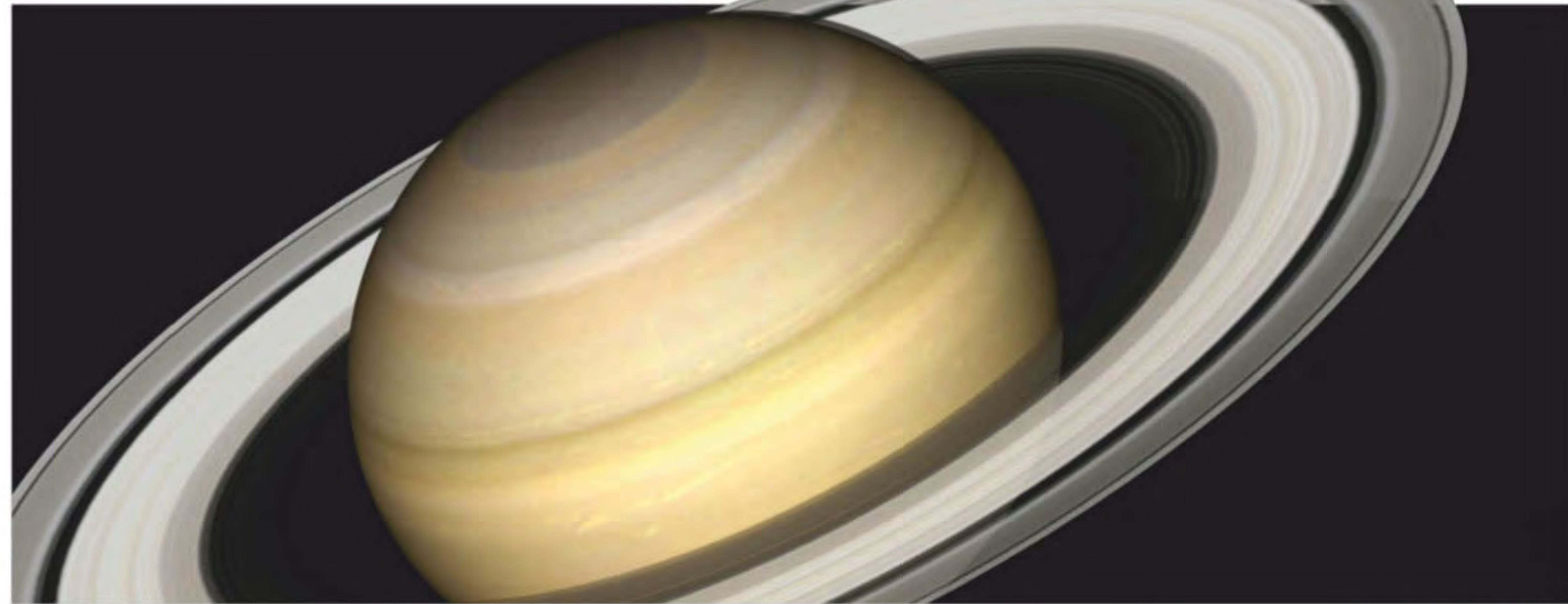
The Cassini spacecraft captured this stunning view of Saturn and its rings on 25 April 2016
