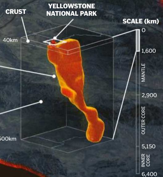
Yellowstone's hot springs are fuelled by the magma chambers below
