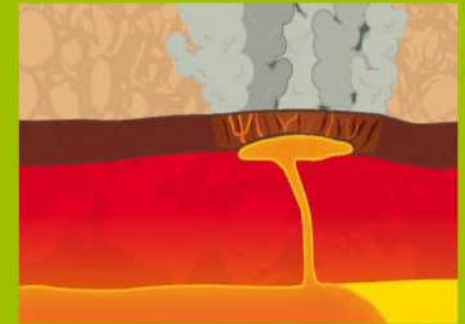
Kilauea is one of the most active volcanoes on Earth, but most of its eruptions are only VEI 0-1
