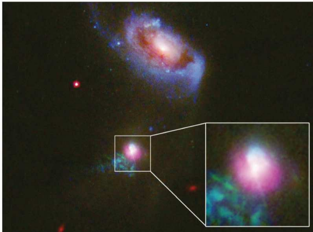
The burping galaxy (bottom) and its companion (top) are seen here in X-ray and optical light
