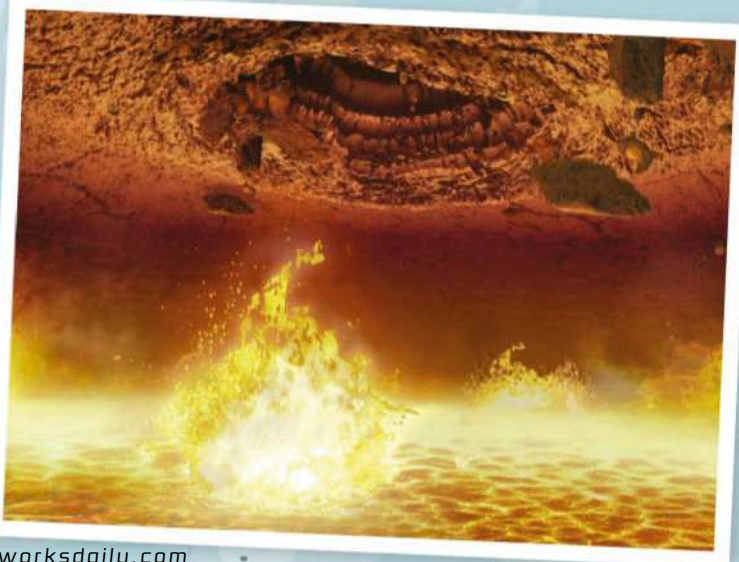
The heart of a supervolcano contains a bubbling magma chamber
