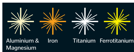
Powdered metals react with oxygen to produce metal oxides, which burn with specific colours
