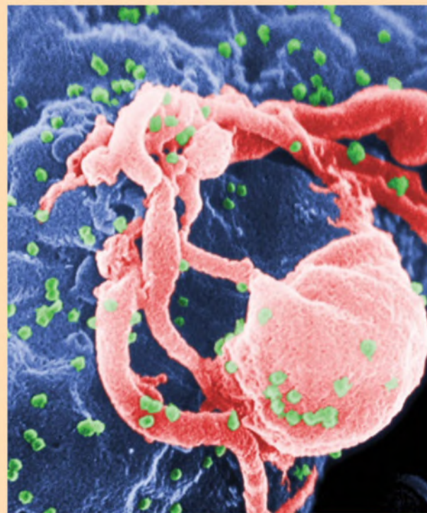
Scanning electron micrograph of HIV-1 budding (in green) from cultured lymphocyte. This image has been coloured to highlight the most important features. Multiple round bumps on the cell surface represent sites of assembly and budding of virions.
